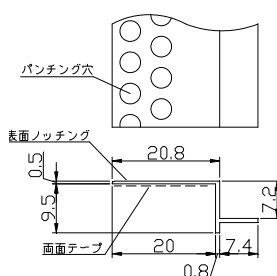
●振動吸収目地CT3(L)
