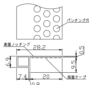
●振動吸収目地CT3(R)
